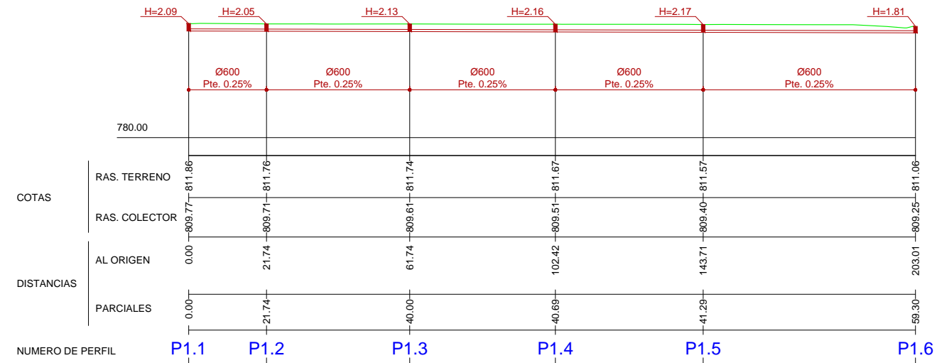
COLECTOR 1
