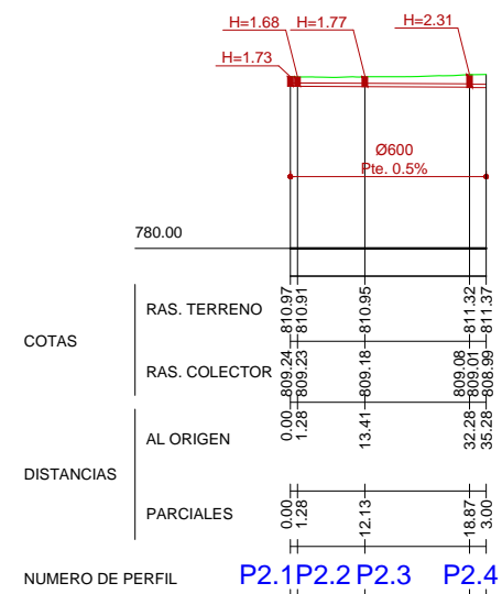
COLECTOR 2
